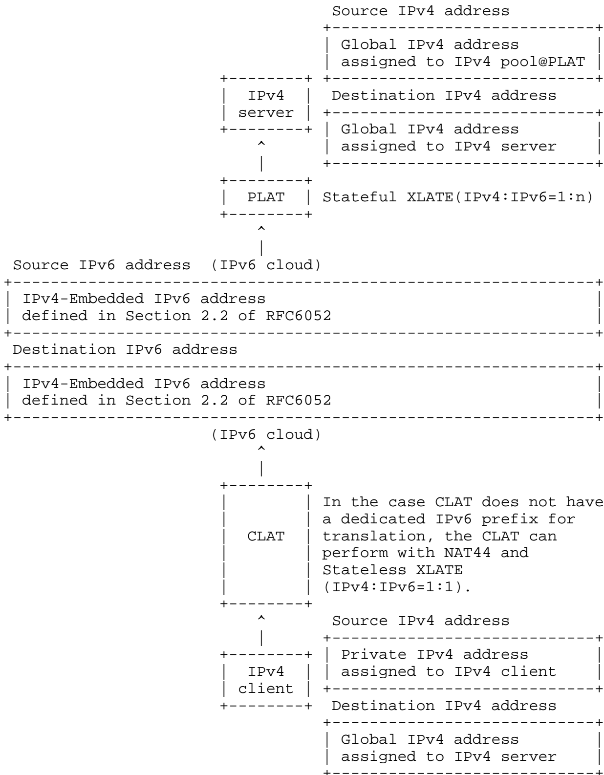
Case of enabling NAT44 and stateless XLATE on CLAT
